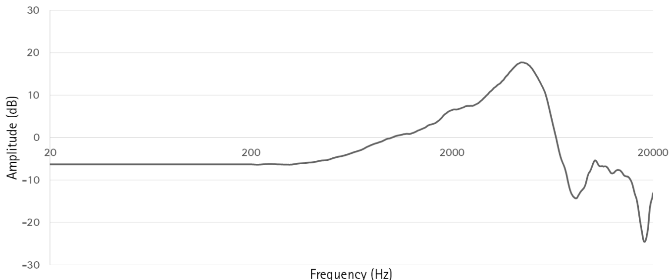
Frequency response
