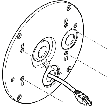
AXIS Q35-V/VE
