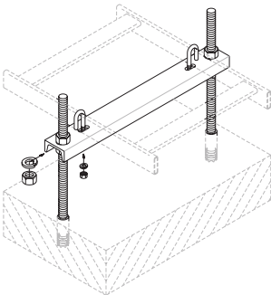
1/2 Pair Shown
