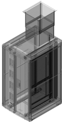
Side-To-Top Airflow - Example P/N: NX5X-XX4X-X5X-X Combine Side Intake Duct with Solid Metal Rear Door with Perforated Insert and Vertical Exhaust Duct Top Panel. Side airflow; top exhaust.
