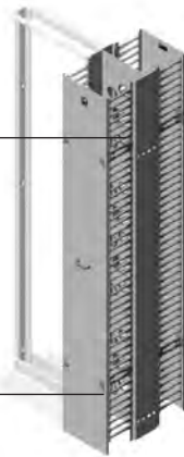
Extended fingers of MCS-EFX
