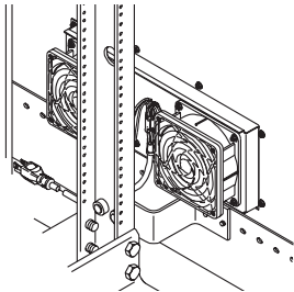
Single Rack Enclosure
