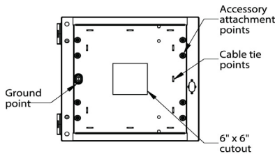
Rear Panel View (Interior Detail)
