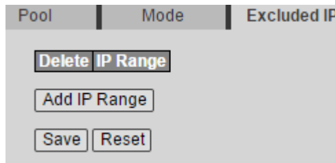
Figure 4-16 Excluded IP
