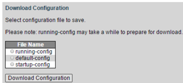
Figure 4-130 Download configuration
