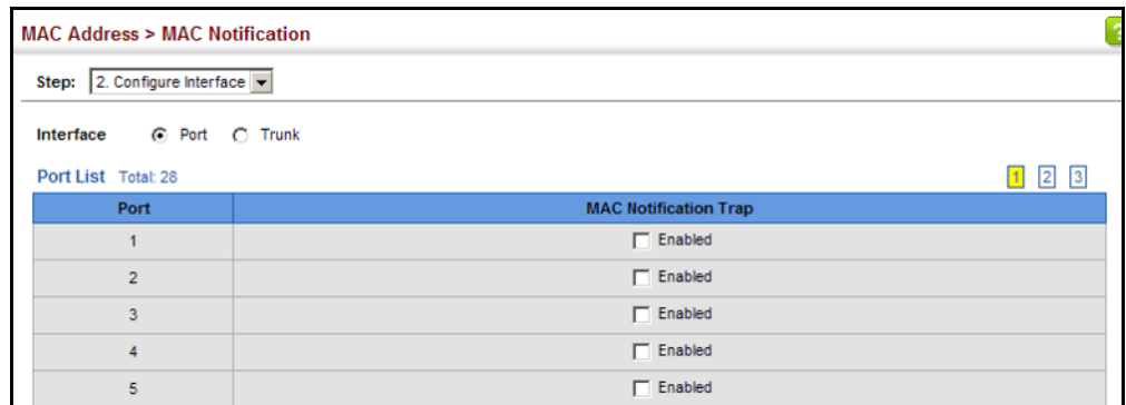
Figure 91: Issuing MAC Address Traps (Interface Configuration)
