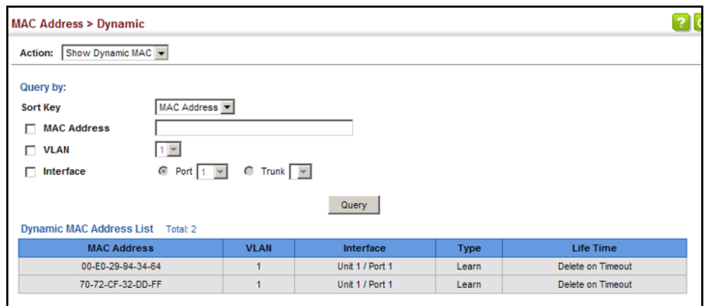
Figure 88: Displaying the Dynamic MAC Address Table
