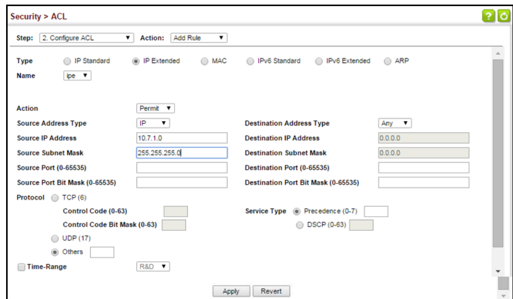
Figure 172: Configuring an Extended IPv4 ACL
