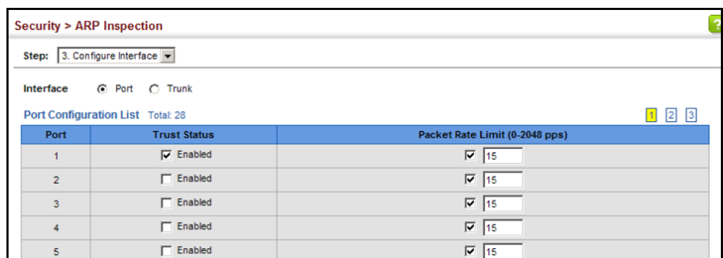
Figure 181: Configuring Interface Settings for ARP Inspection
