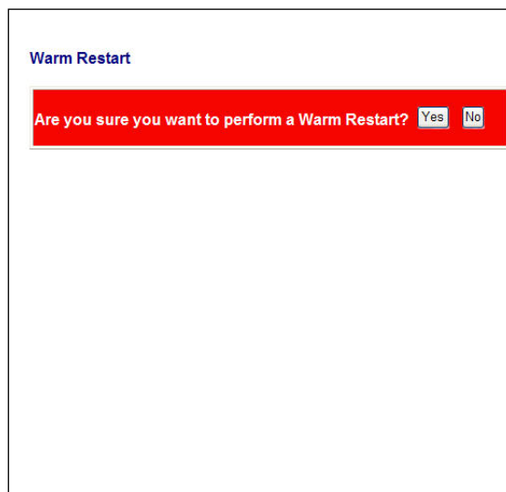
Fig. 4-34 Warm Restart
