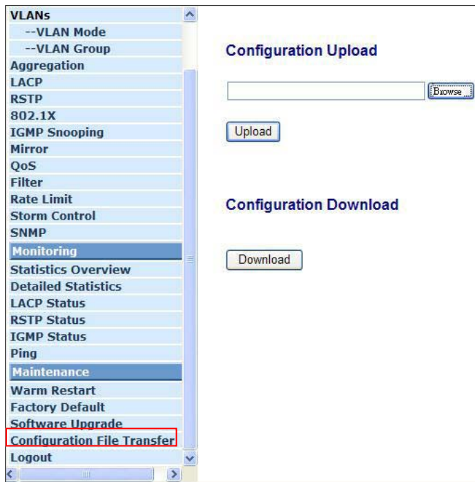
Fig. 4-37 Configuration Upload/Download
