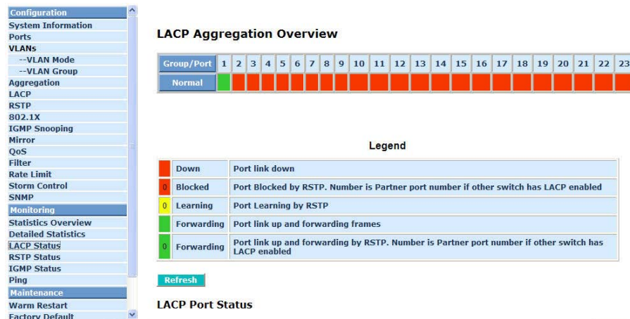
Fig. 4-30 LACP Status
