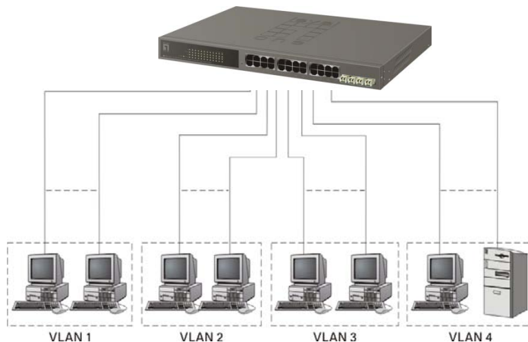
Fig. 2-3 Port-based VLAN Diagram
