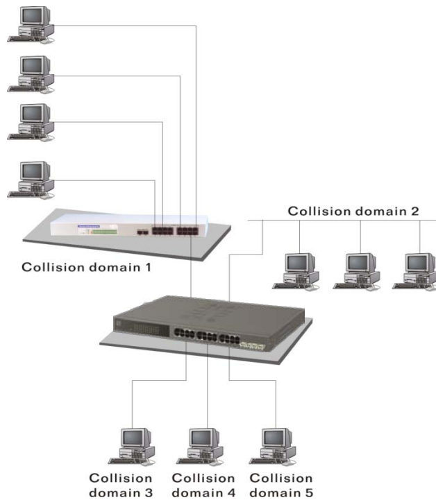
Fig.3-5 Collision Domain
