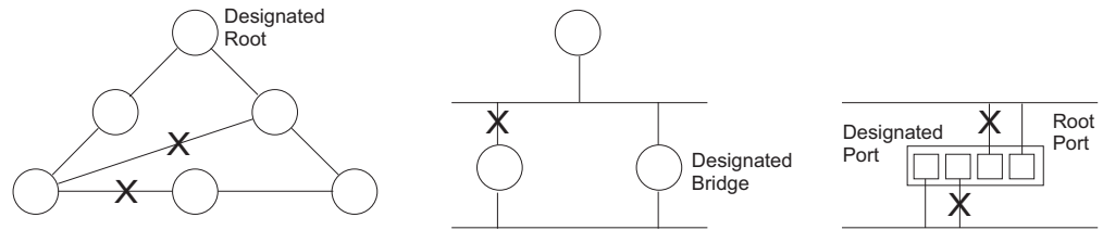
Figure 112: STP Root Ports and Designated Ports
