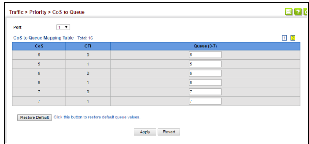
Figure 143: Configuring CoS to Queue Mapping
