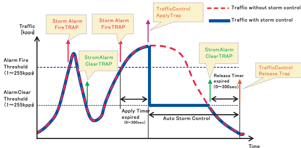
Figure 134: Storm Control by Limiting the Traffic Rate
