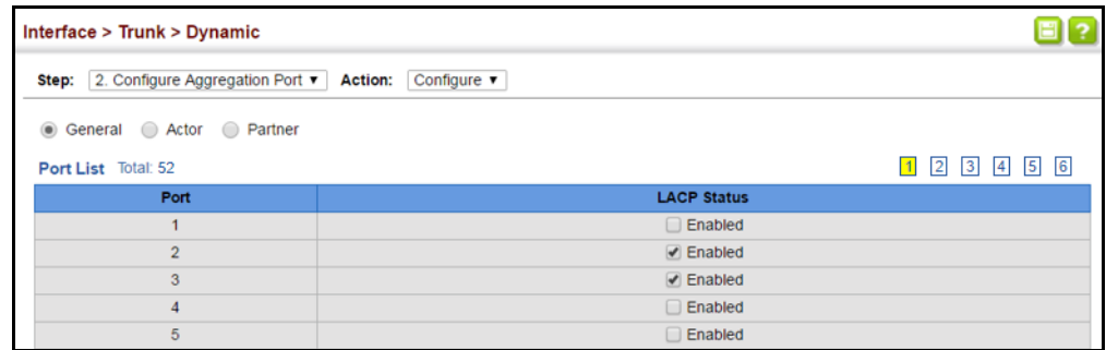
Figure 50: Enabling LACP on a Port
