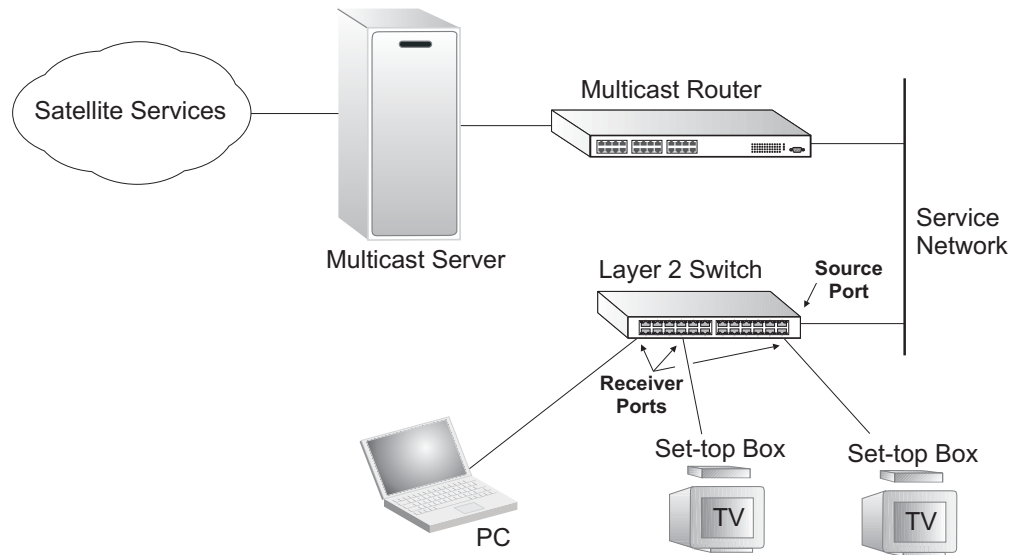
Figure 386: MVR Concept
