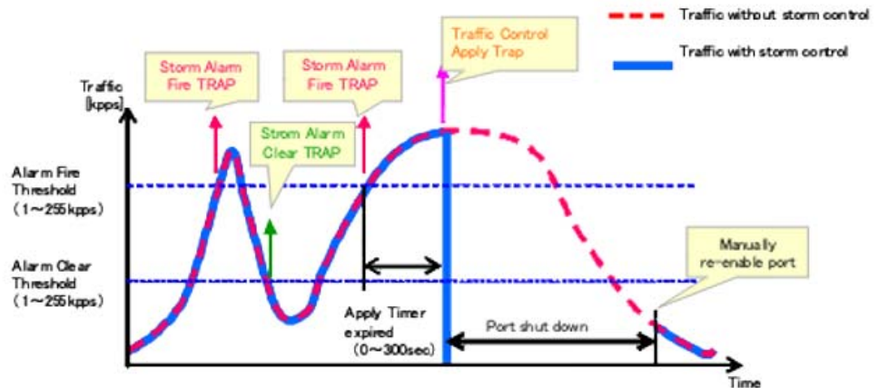
Figure 135: Storm Control by Shutting Down a Port
