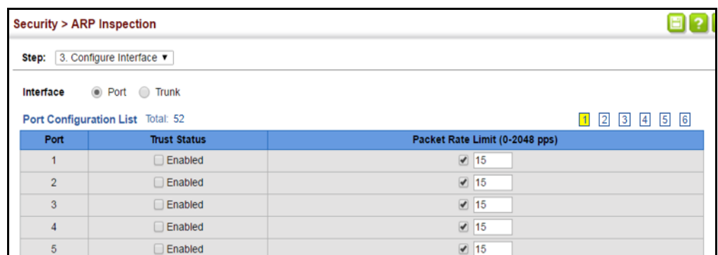
Figure 232: Configuring Interface Settings for ARP Inspection
