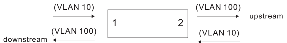
Figure 101: Configuring VLAN Translation
