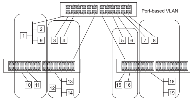
Figure 75: Using GVRP
