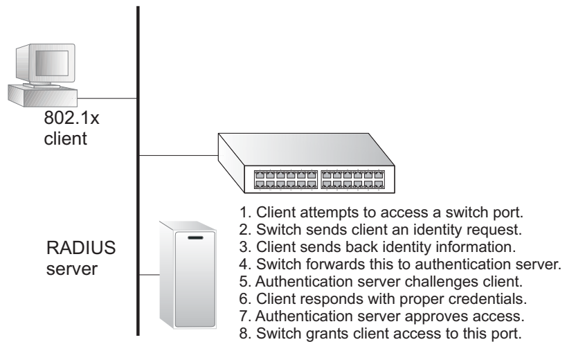
Figure 207: Configuring Port Authentication
