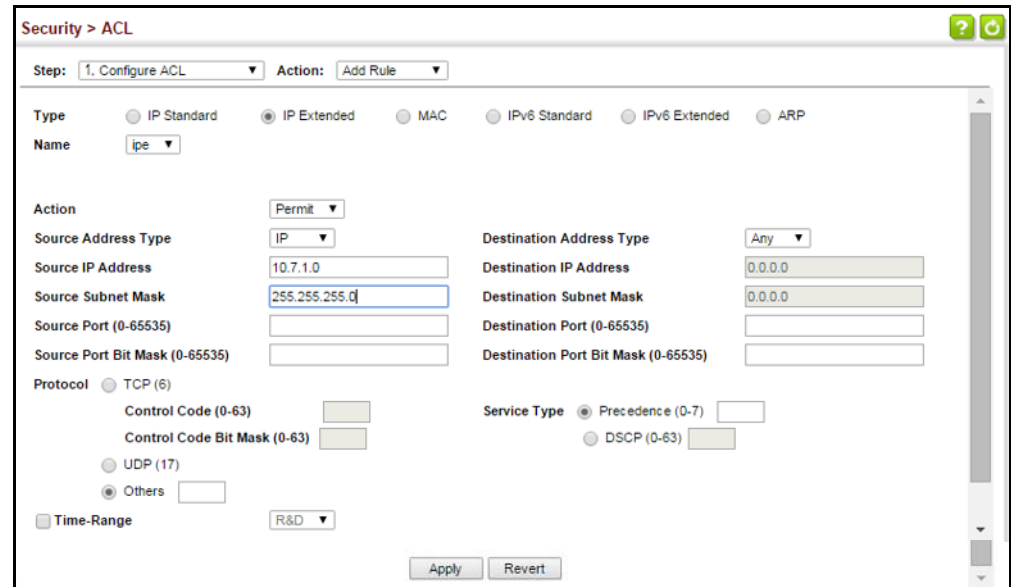
Figure 197: Configuring an Extended IPv4 ACL
