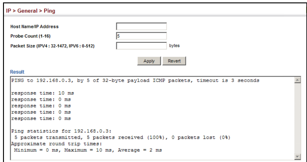
Figure 441: Pinging a Network Device
