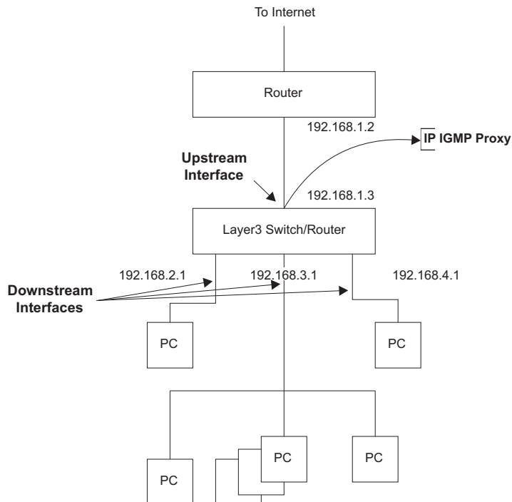
Figure 365: IGMP Proxy Routing
