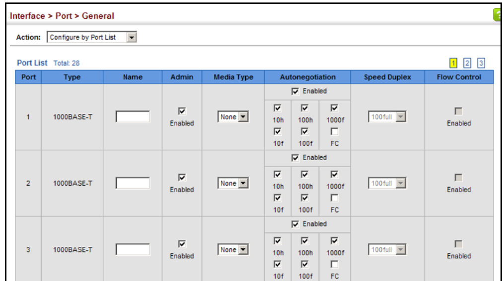
Figure 32: Configuring Connections by Port List
