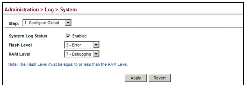
Figure 237: Configuring Settings for System Memory Logs
