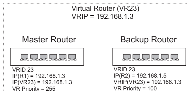
Figure 454: Master Virtual Router with Backup Routers
