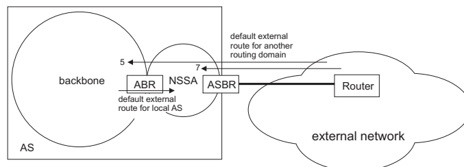
Figure 492: OSPF NSSA
