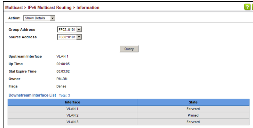
Figure 521: Displaying Detailed Entries from IPv6 Multicast Routing Table
