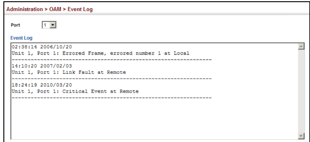
Figure 329: Displaying the OAM Event Log
