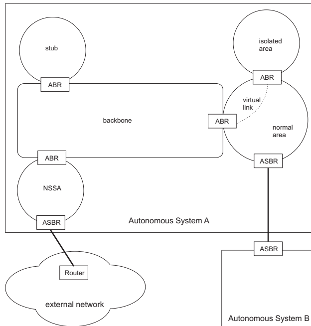
Figure 482: Configuring OSPF
