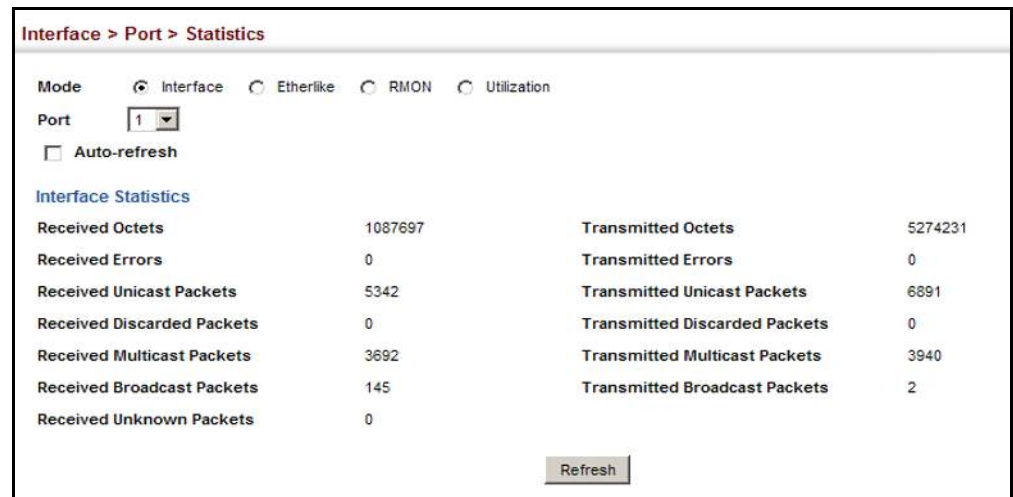
Figure 34: Showing Port Statistics (Table)
