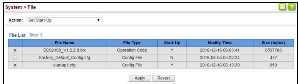
Figure 9: Setting Start-Up Files
