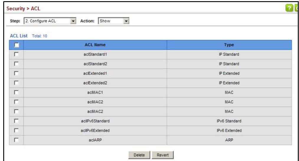
Figure 177: Showing a List of ACLs
