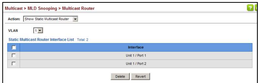
Figure 303: Showing Static Interfaces Attached an IPv6 Multicast Router
