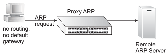
Figure 324: Proxy ARP
