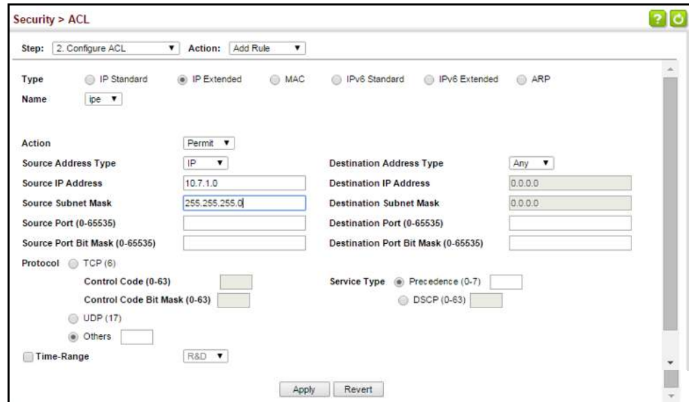
Figure 179: Configuring an Extended IPv4 ACL
