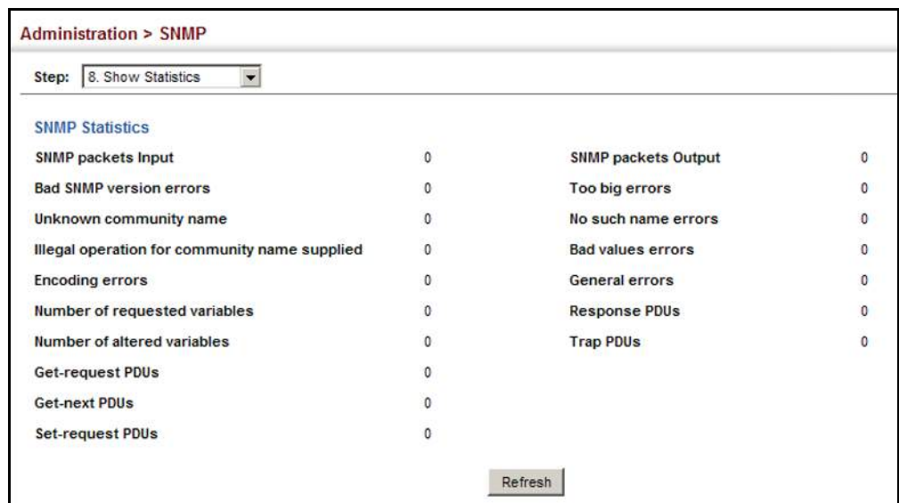
Figure 248: Showing SNMP Statistics
