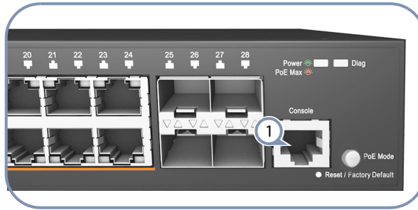
Figure 25: Console Port
