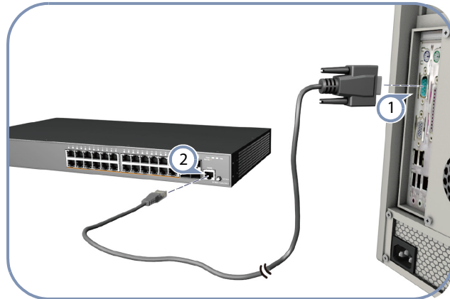
Figure 26: Console Port Connection
