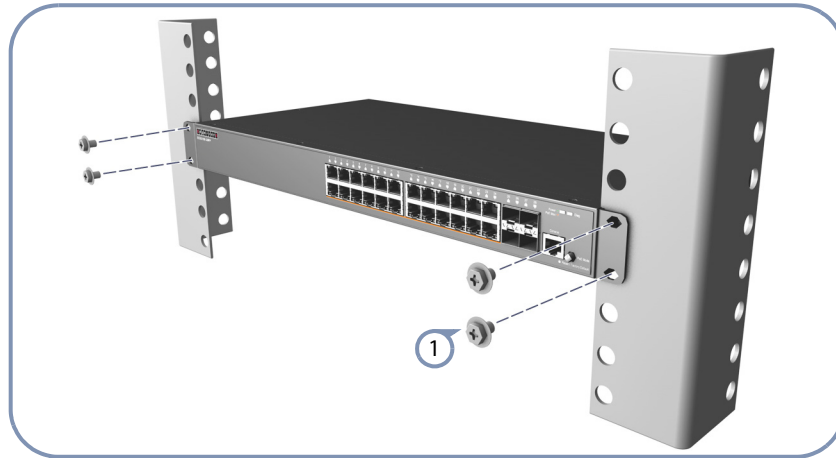
Figure 13: Installing the Switch in a Rack
