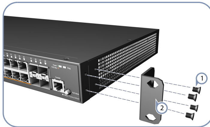
Figure 12: Attaching the Brackets
