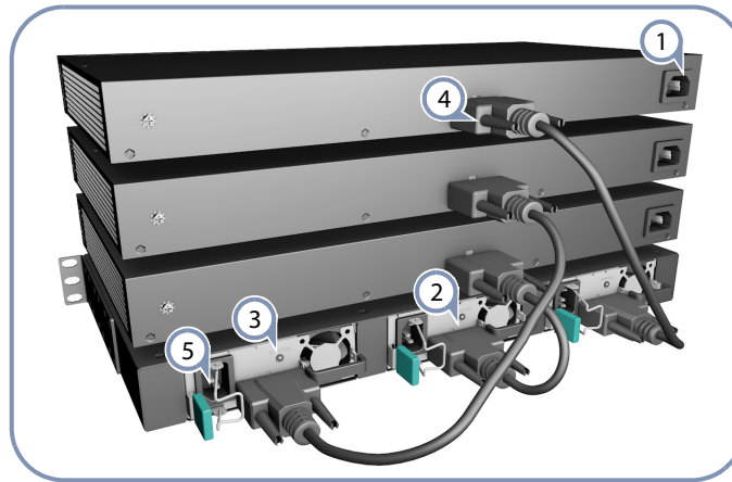
1 External Power Supply—EPS460W
