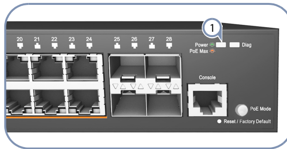
Figure 24: System LEDs
