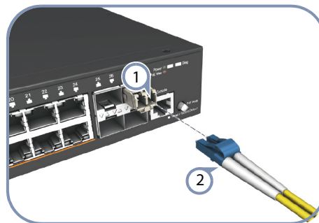
Figure 23: Making a Connection to an SFP/SFP+ Port
