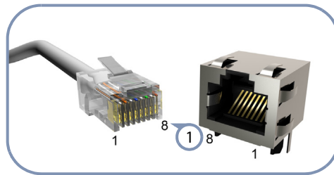
1 RJ-45 Pin Numbers
