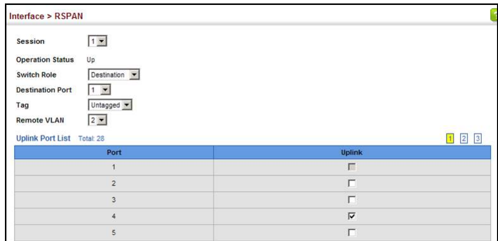
Figure 66: Configuring Remote Port Mirroring (Destination)
