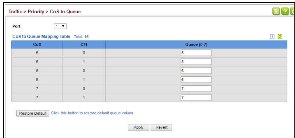
Figure 135: Configuring CoS to Queue Mapping
