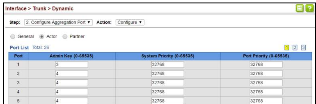
Figure 51: Configuring LACP Parameters on a Port
