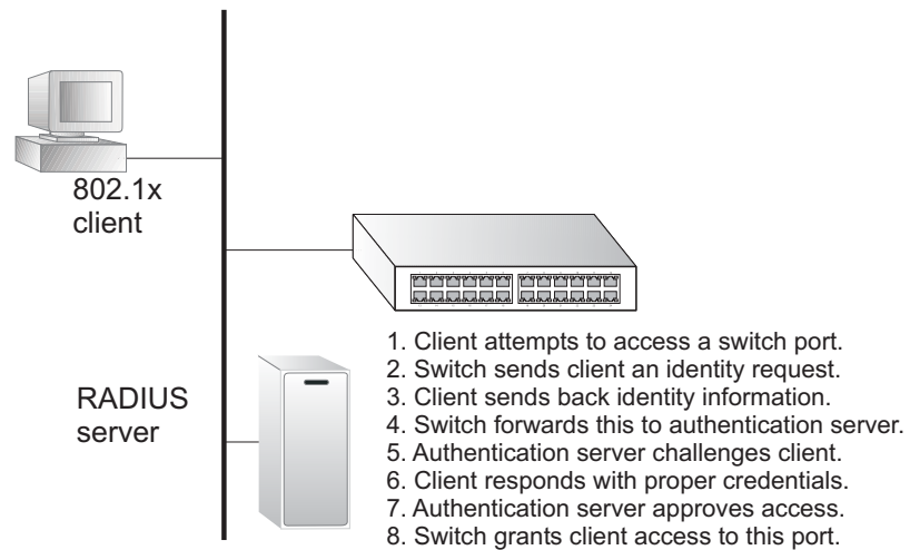
Figure 199: Configuring Port Authentication
