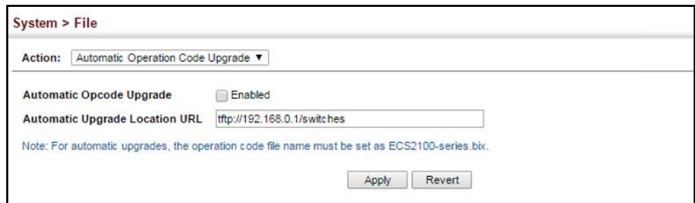
Figure 10: Configuring Automatic Code Upgrade
