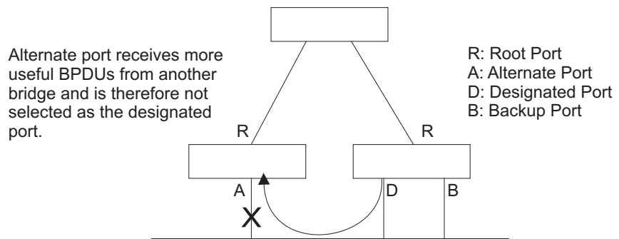
Figure 118: STA Port Roles
