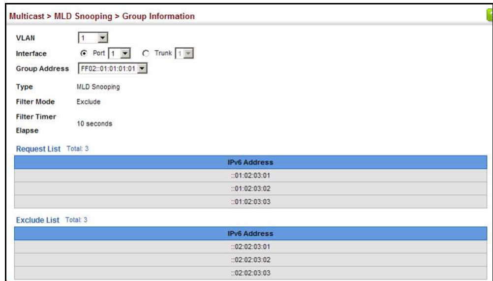
Figure 358: Showing IPv6 Multicast Services and Corresponding Sources
