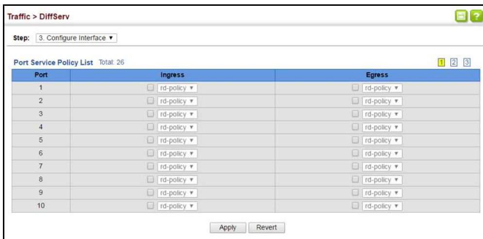
Figure 145: Attaching a Policy Map to a Port
