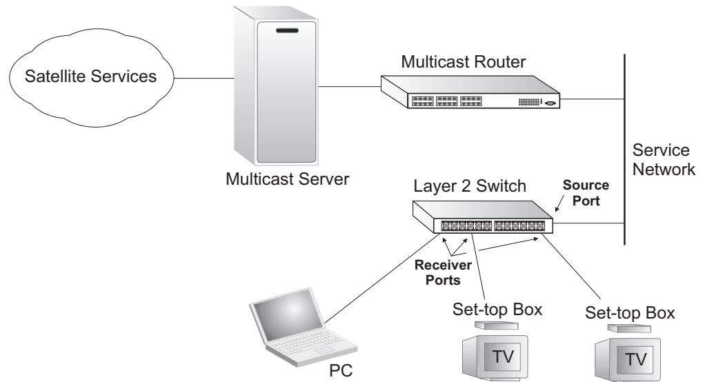
Figure 372: MVR Concept
