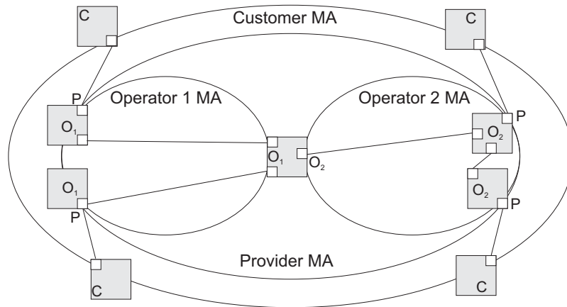
Figure 298: Multiple CFM Maintenance Domains
