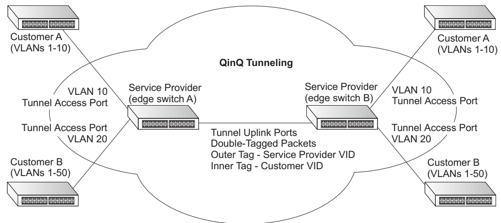
Figure 85: QinQ Operational Concept
