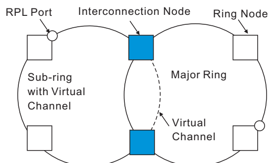
Figure 290: Sub-ring with Virtual Channel
