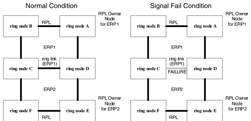
Figure 288: Ring Interconnection Architecture (Multi-ring/Ladder Network)
