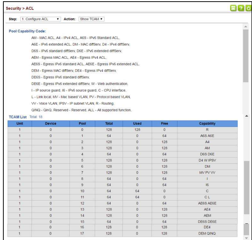
Figure 185: Showing TCAM Utilization
