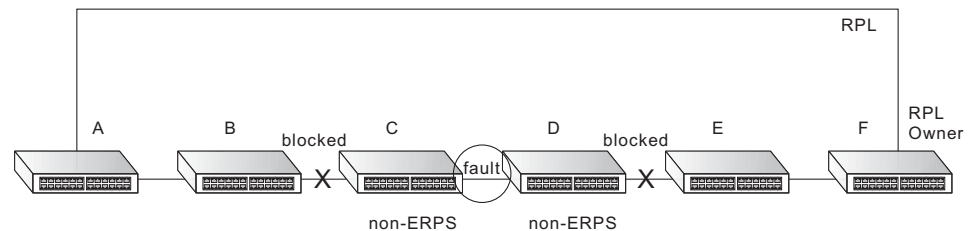
Figure 292: Non-ERPS Device Protection
