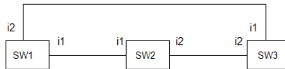
Figure 116: Determining the Root Port
