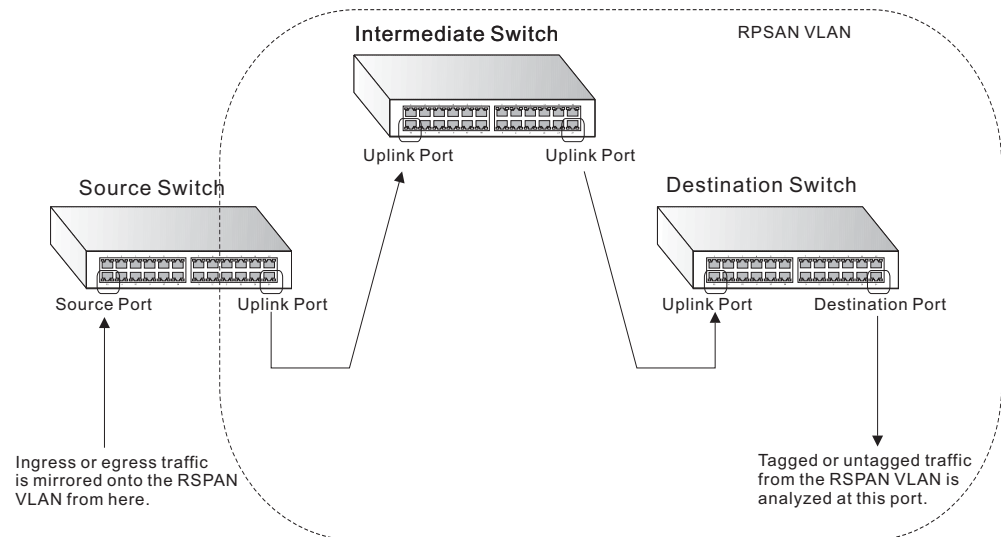
Figure 62: Configuring Remote Port Mirroring
