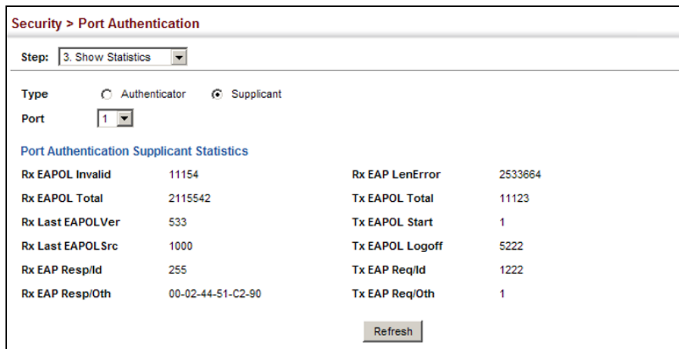
Figure 223: Showing Statistics for 802.1X Port Supplicant
