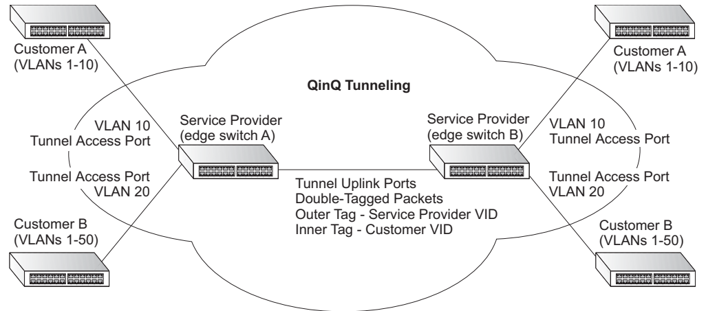
Figure 87: QinQ Operational Concept
