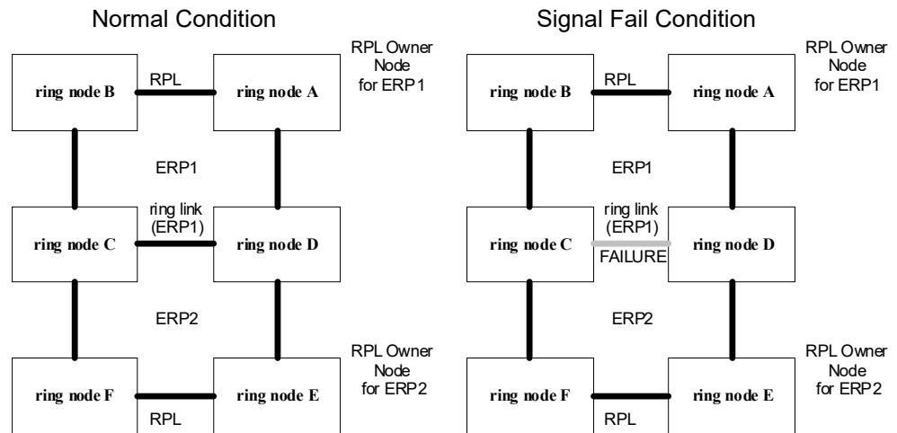
Figure 304: Ring Interconnection Architecture (Multi-ring/Ladder Network)
