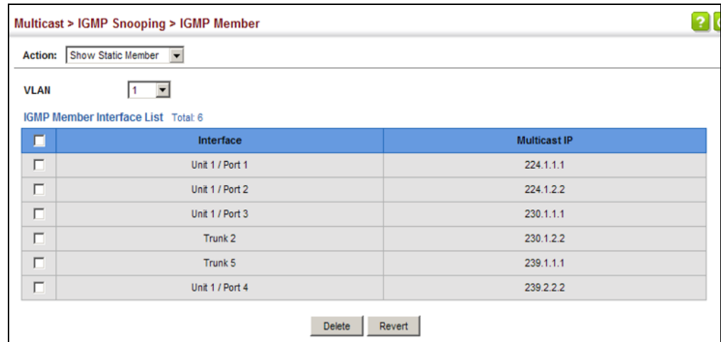
Figure 328: Showing Static Interfaces Assigned to a Multicast Service
