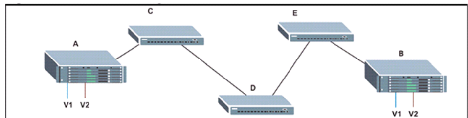
Figure 73: Configuring VLAN Trunking
