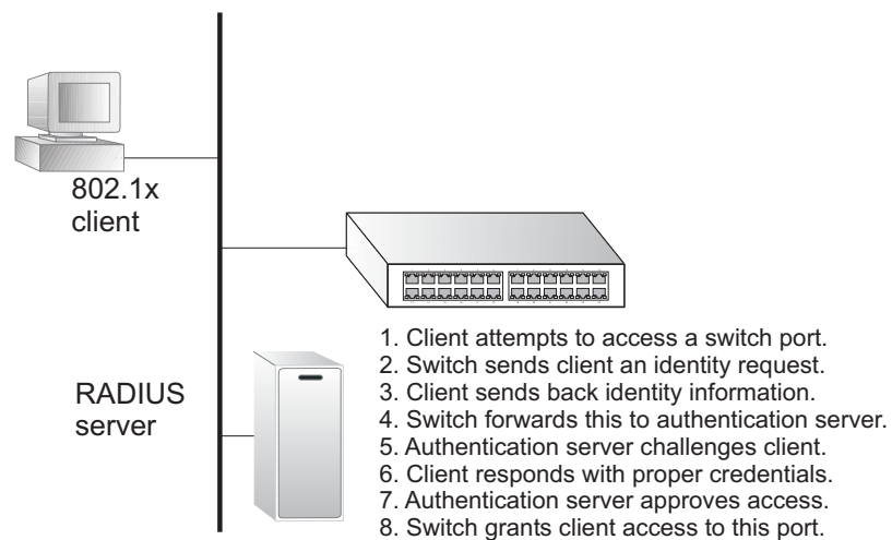
Figure 218: Configuring Port Authentication
