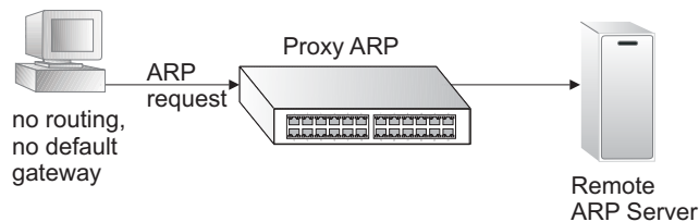
Figure 381: Proxy ARP
