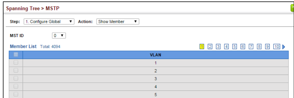
Figure 134: Displaying Members of an MST Instance
