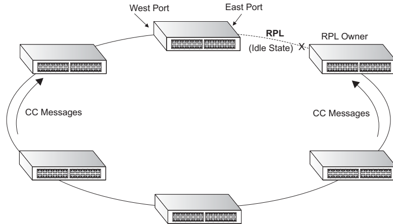
Figure 303: ERPS Ring Components
