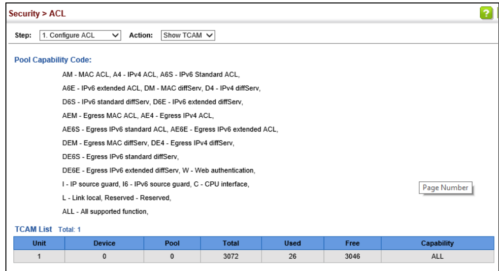
Figure 204: Showing TCAM Utilization
