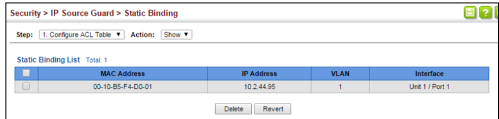
Figure 237: Displaying Static Bindings for IPv4 Source Guard
