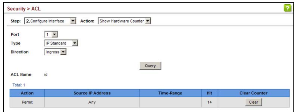
Figure 214: Showing ACL Statistics
