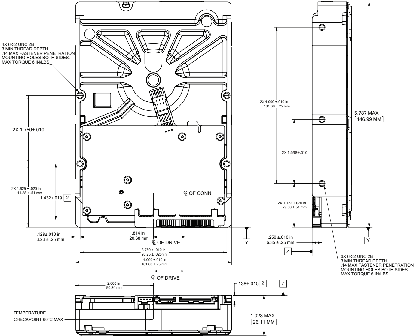
Figure 4 Mounting dimensions (6TB)
