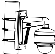
DS-1275ZJ-SUS Vertical Pole Mount
