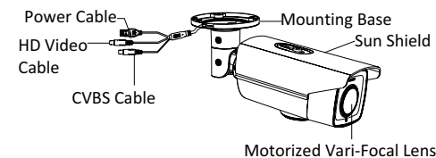
Figure 1-1 Overview of Bullet Camera
