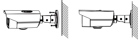
Figure 2-5 Fix the Camera to the Wall
