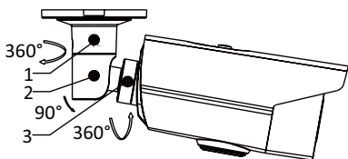
Figure 2-4 3-axis Adjustment
