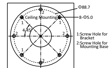
Figure 2-1 Drill Template
