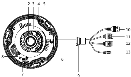
Figure 1-2 Overview of Dome Camera (2)
