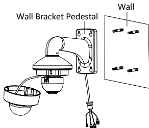
Figure 2-11 Install the Wall Bracket
