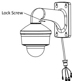
Figure 2-12 Install the Black Liner and Bubble
