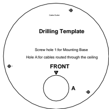
Figure 2-2 Drill Template
