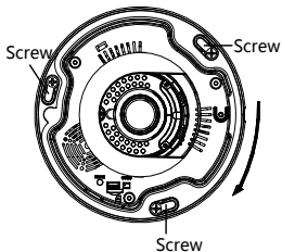
Figure 2-4 Fix the Camera Pedestal
