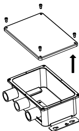
Figure 2-14 Open the Junction Box
