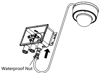
Figure 2-16 Route the Cables
