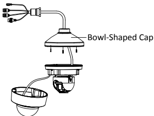
Figure 2-8 Fix the Camera
