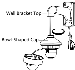
Figure 2-9 Install the Bowl-Shaped Cap
