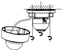
Figure 2-6 Tighten the Three Screws
