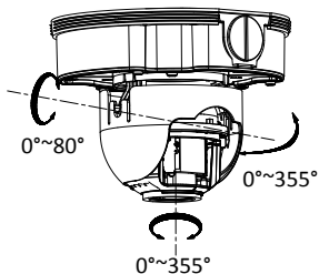
Figure 2-5 3-axis Adjustment
