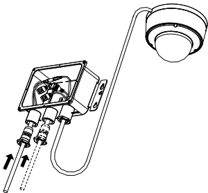
Figure 2-17 Connect the Cables
