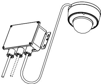
Figure 2-18 Fix the Cover of Junction Box
