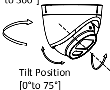
Figure 2-4 3-axis Adjustment
