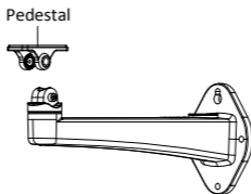
Figure 2-4 Separate Pedestal
