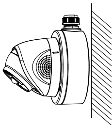
Figure 2-13 Finish the Installation
