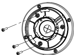
Figure 2-12 Secure Mounting Base on Junction Box's Cover
