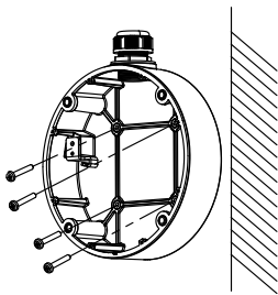
Figure 2-11 Secure the Junction Box's Body
