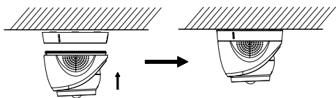
Figure 2-9 Install Camera Back
