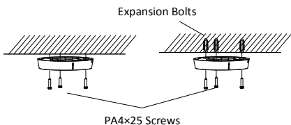
Figure 2-8 Attach Mounting Base to Ceiling
