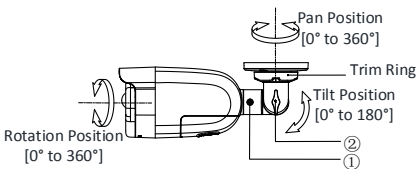
Figure 2-2 3-Axis Adjustment
