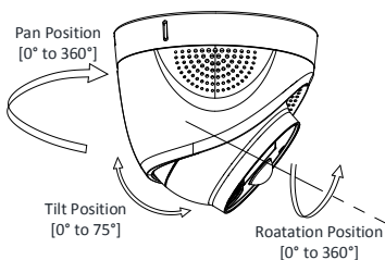
Figure 2-10 3-Axis Adjustment
