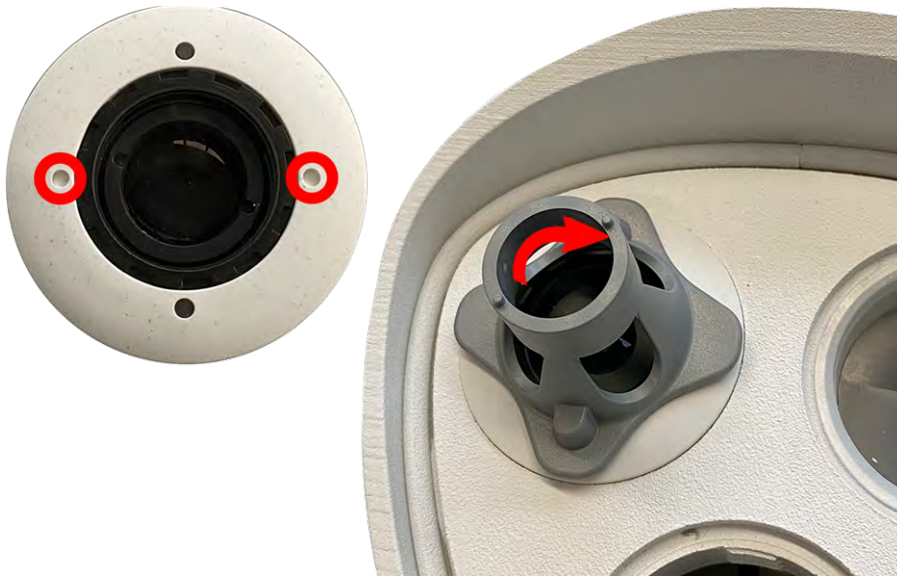
Fig. 11: Lock the sensor module
