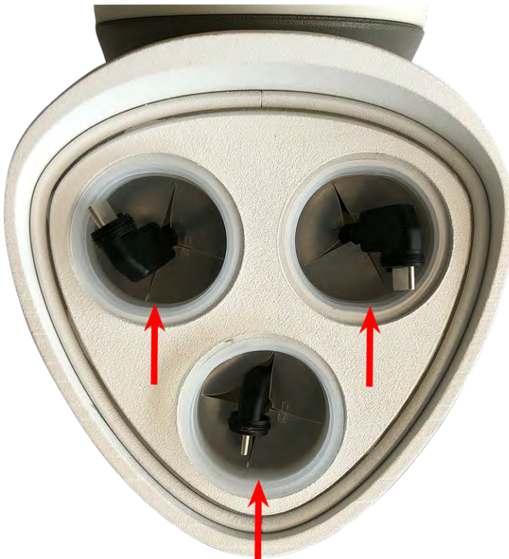
Fig. 26: Remove the transport plugs
