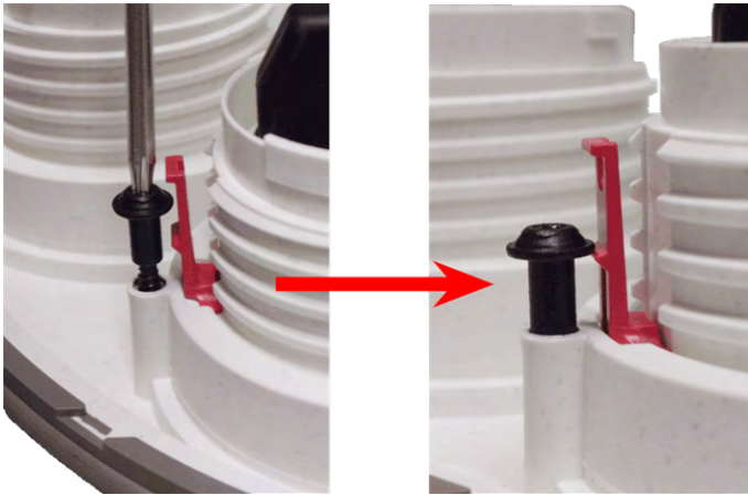
Fig. 17: Use screw to lock security clip in place
