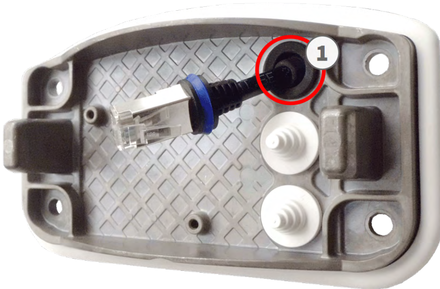
Fig. 34: Prepare the mounting plate
