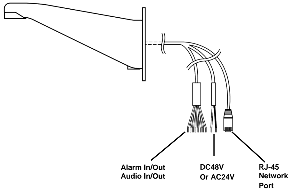
FIGURE 2-2: ROUTING THE CABLES
