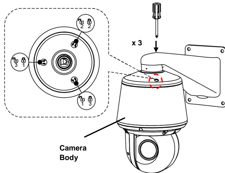
FIGURE 2-5: LOOSENING THE PENDANT CAP
