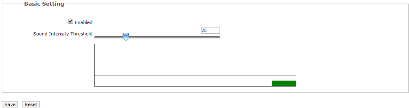
FIGURE 2-45: AUDIO DETECTION
