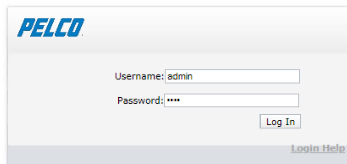
FIGURE 1-2: LOGIN WINDOW
