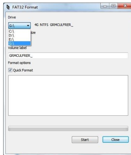
FIGURE 2-55: FAT32 FORMAT
