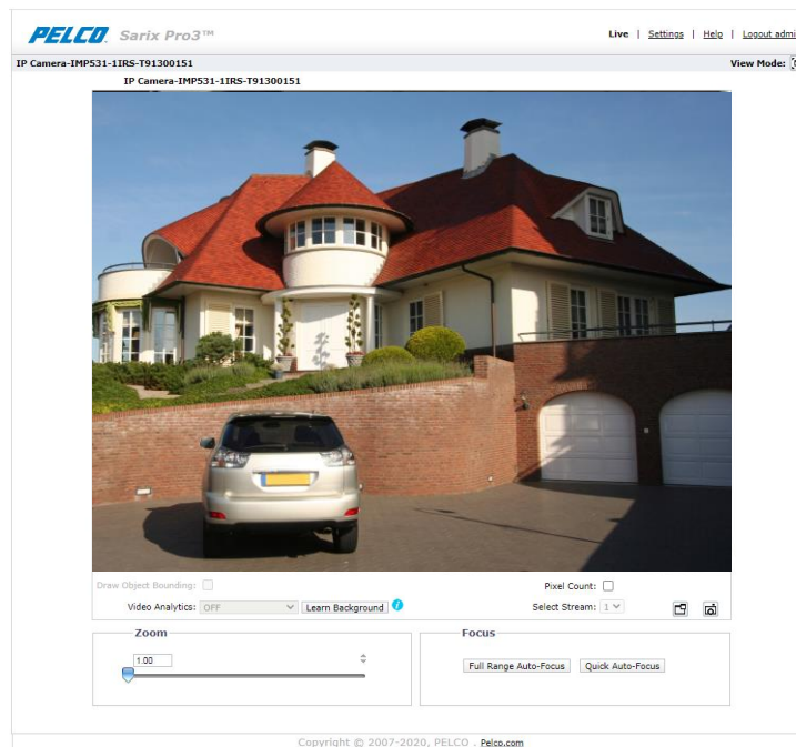
FIGURE 2-1: LIVE VIEW
