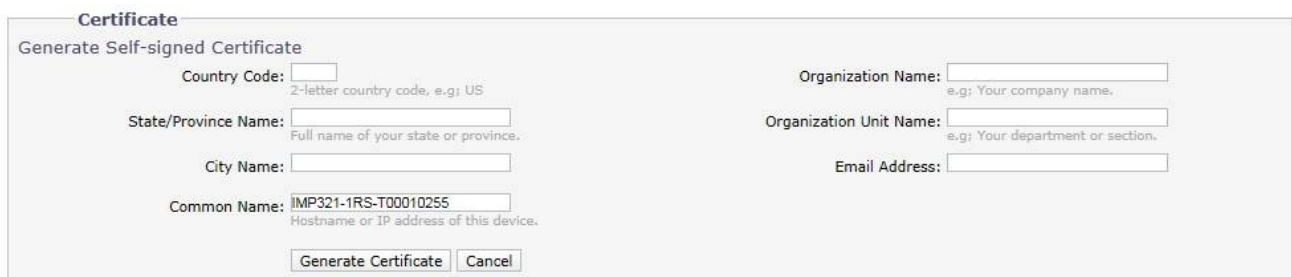
FIGURE 2-17: GENERATING SELF-SIGNED CERTIFICATE CONFIGURATION
