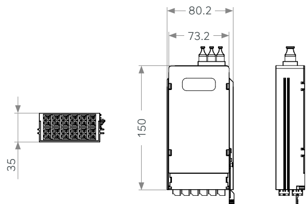
MD-24F MPO-LC-Kassette
