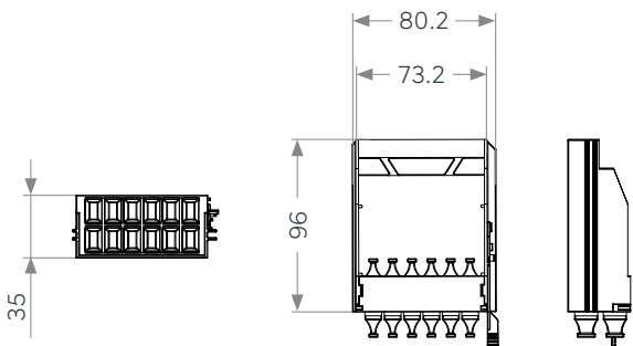
MD-12 Port MPO Passthrough Cassette
