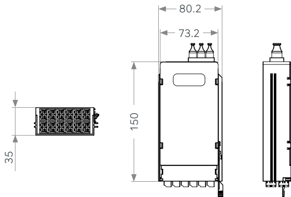
MD-24F MPO-LC Cassette
