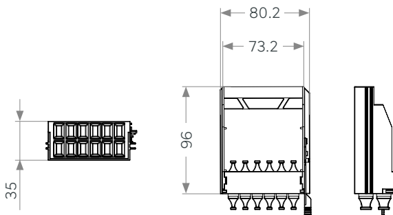
Cassette MD-12 Port MPO Passthrough
