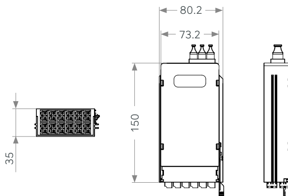
Kaseta MD-24F MPO-LC
