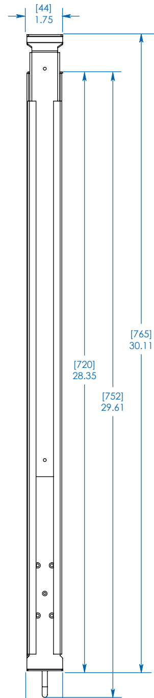
SIDE VIEW
