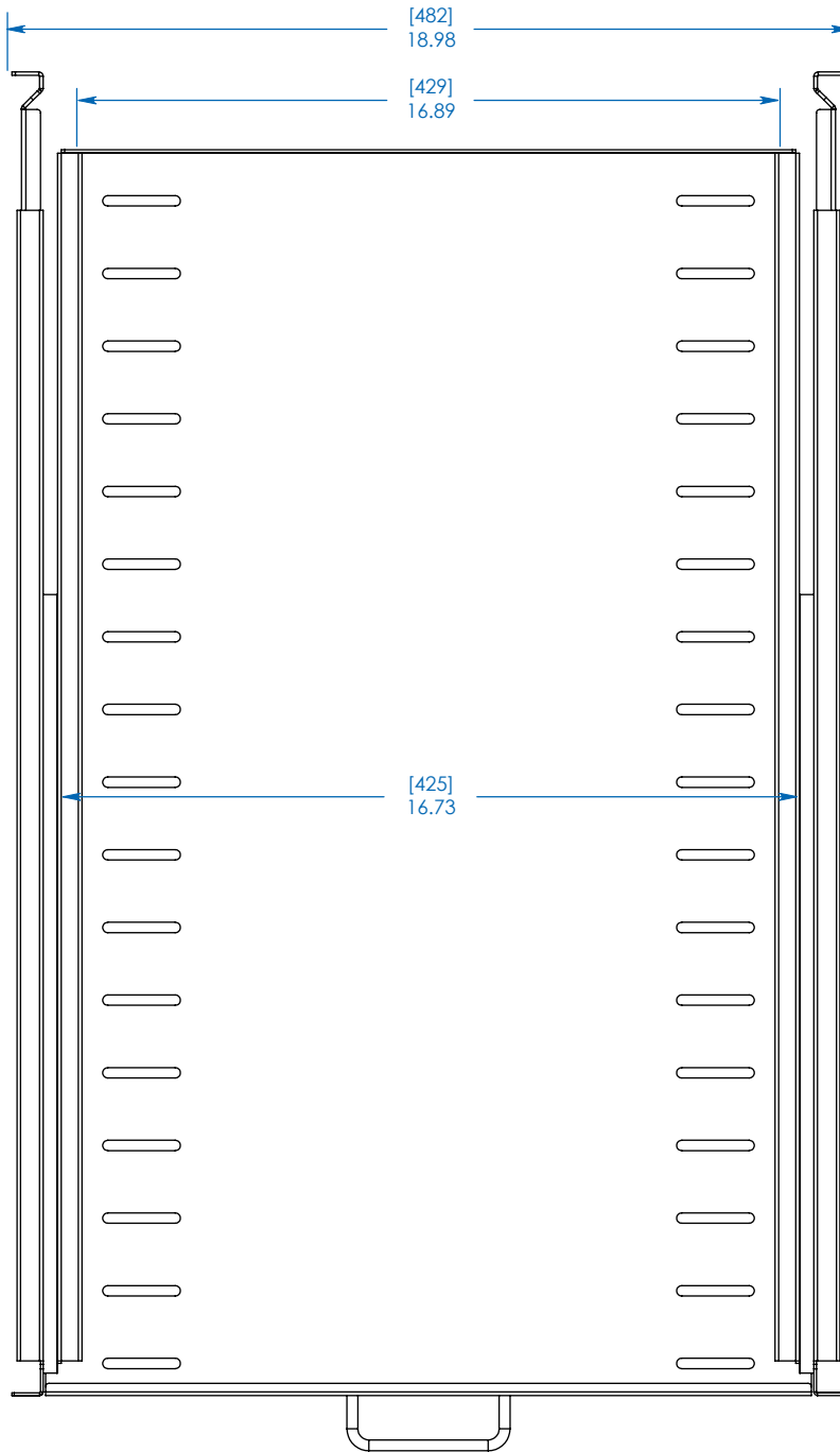
TOP VIEW
