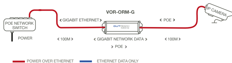
Diagram 1. A single OUTREACH Max G doubles the cable range to a POE IP Camera. Each cable segment can be up to 100 metres.
